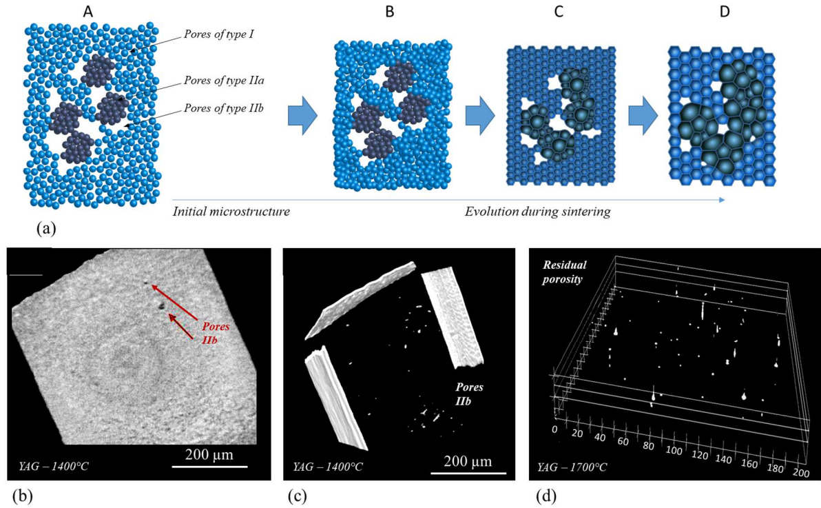
Figure 14: Microstructure evolution model for the densification of different types of pores: green part (A), pore densification of smaller size (type I and IIa) at low temperature accompanied by moderate grain growth (B and C), densification of the larger pores (type IIb) (D) which become unstable under the effect of rapid granular growth at high temperature (a). X-ray microtomography micrograph showing large pores of type IIb in a YAG sample shaped by PSC ( sample S4 ) and vacuum-fired at 1400°C (i.e. at intermediate stage of sintering, \rho = 75\% ), 2D cut in (b) and 3D view after segmentation in (c). Confocal laser scanning microscopy showing residual porosity in 3D in transparent YAG sample shaped by PSC ( sample S4 ) and vacuum-fired at 1700°C (i.e. at final stage of sintering, \rho > 99.9\% ).
